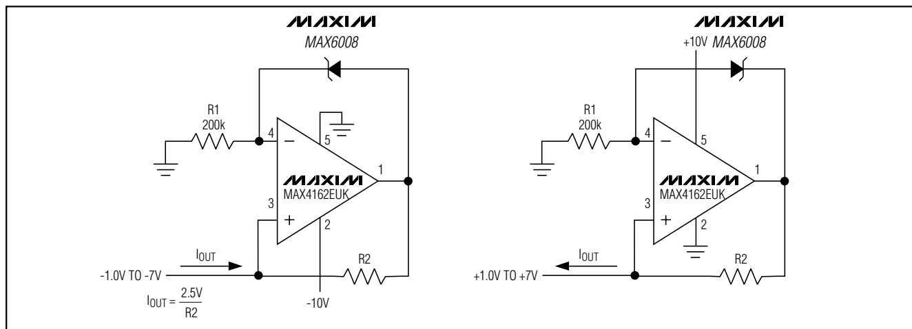
Figure 2. Precision 1 \mu A to 1mA Current Sources
